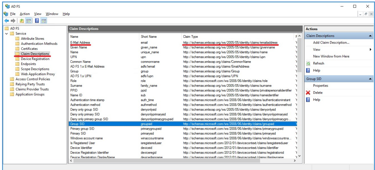
Picture 151. Outgoing claim type
