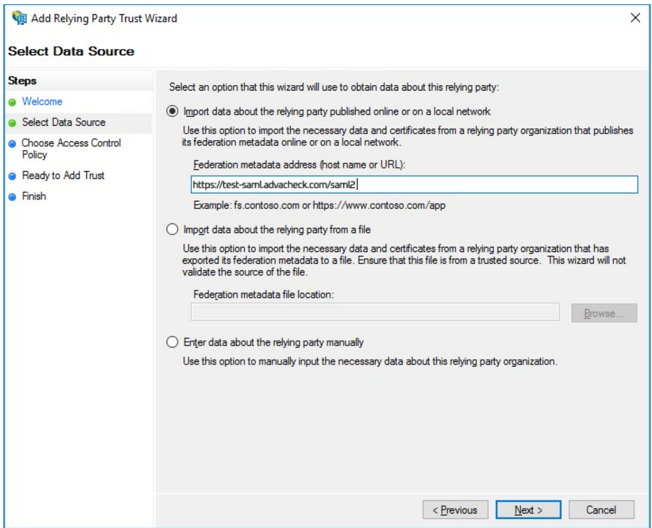
Picture 144. Selecting URL data entry
