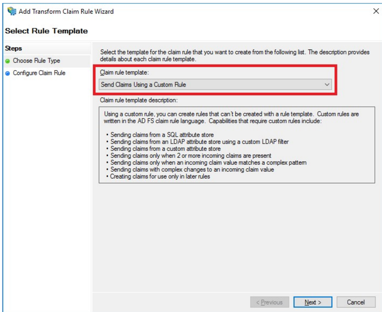
Picture 153. Choosing a template
