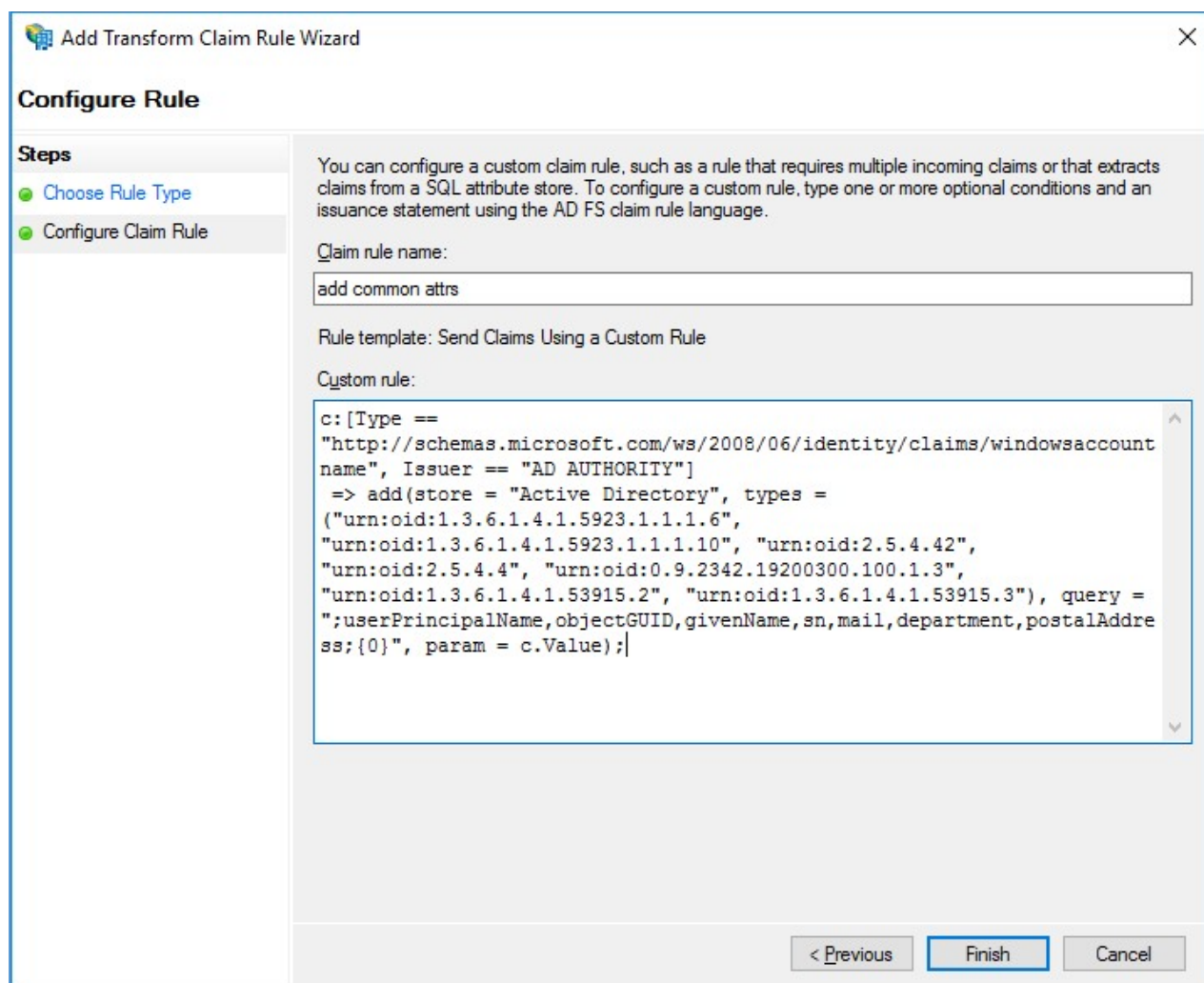
Picture 154. Choosing a template
