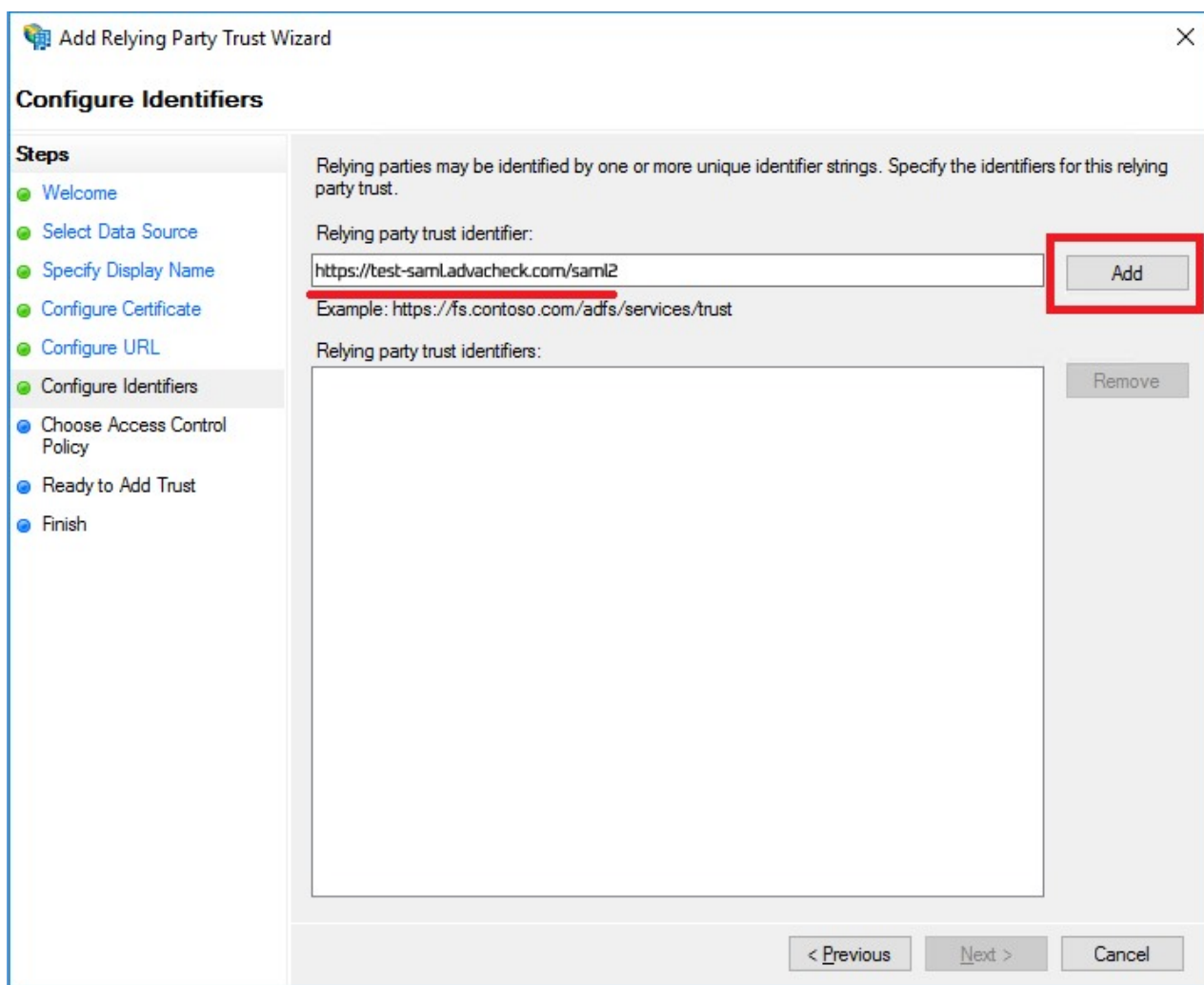
Picture 141. Entering SP ID
