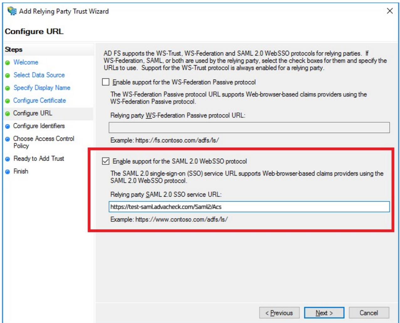
Picture 140. Enabling SAML protocol support
